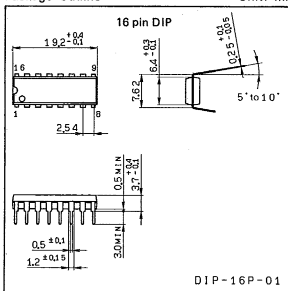
Package Outline
